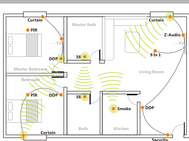
D: For Semi-Retrofit Installation
